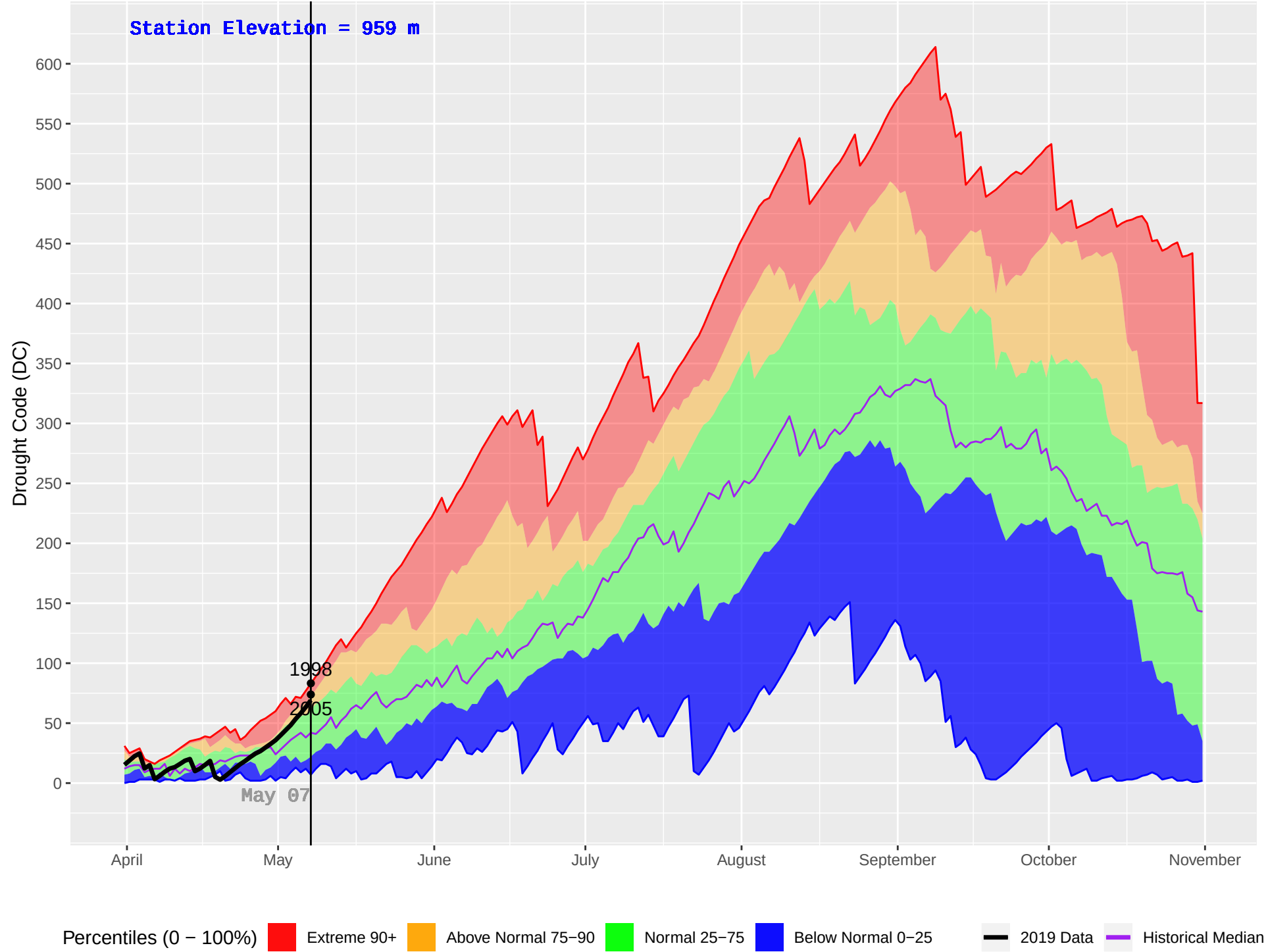
WELLS GRAY (266) : Historical (1994–2018) and Current (2019) Daily Drought Code (DC)
