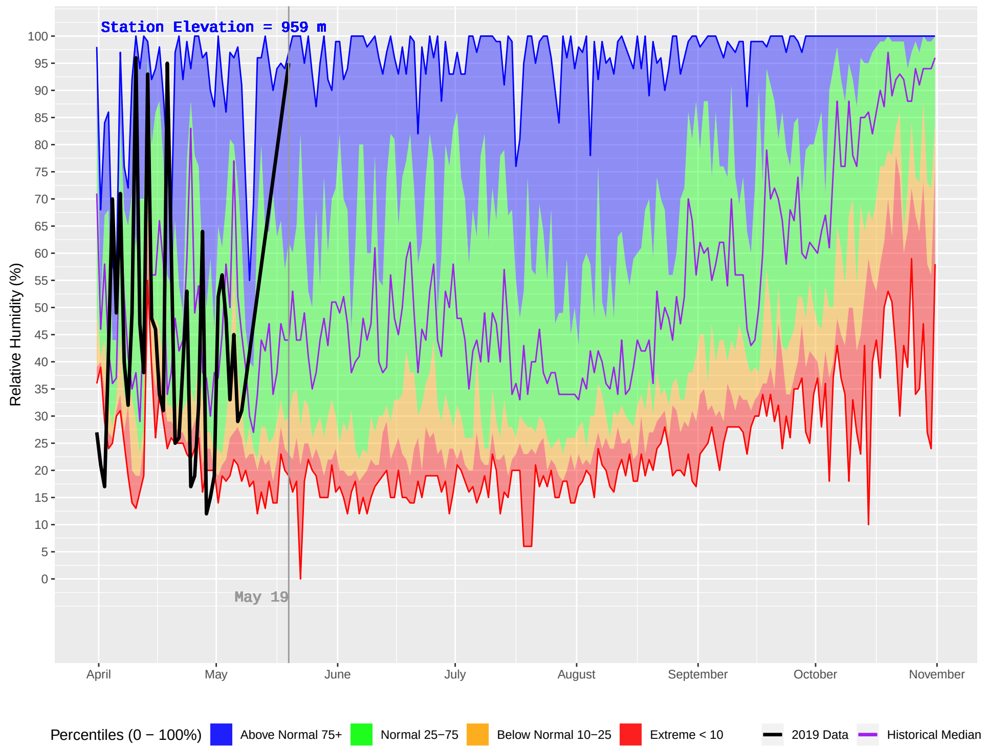
WELLS GRAY (266) : Historical (1994–2018) and Current (2019) Daily Relative Humidity
