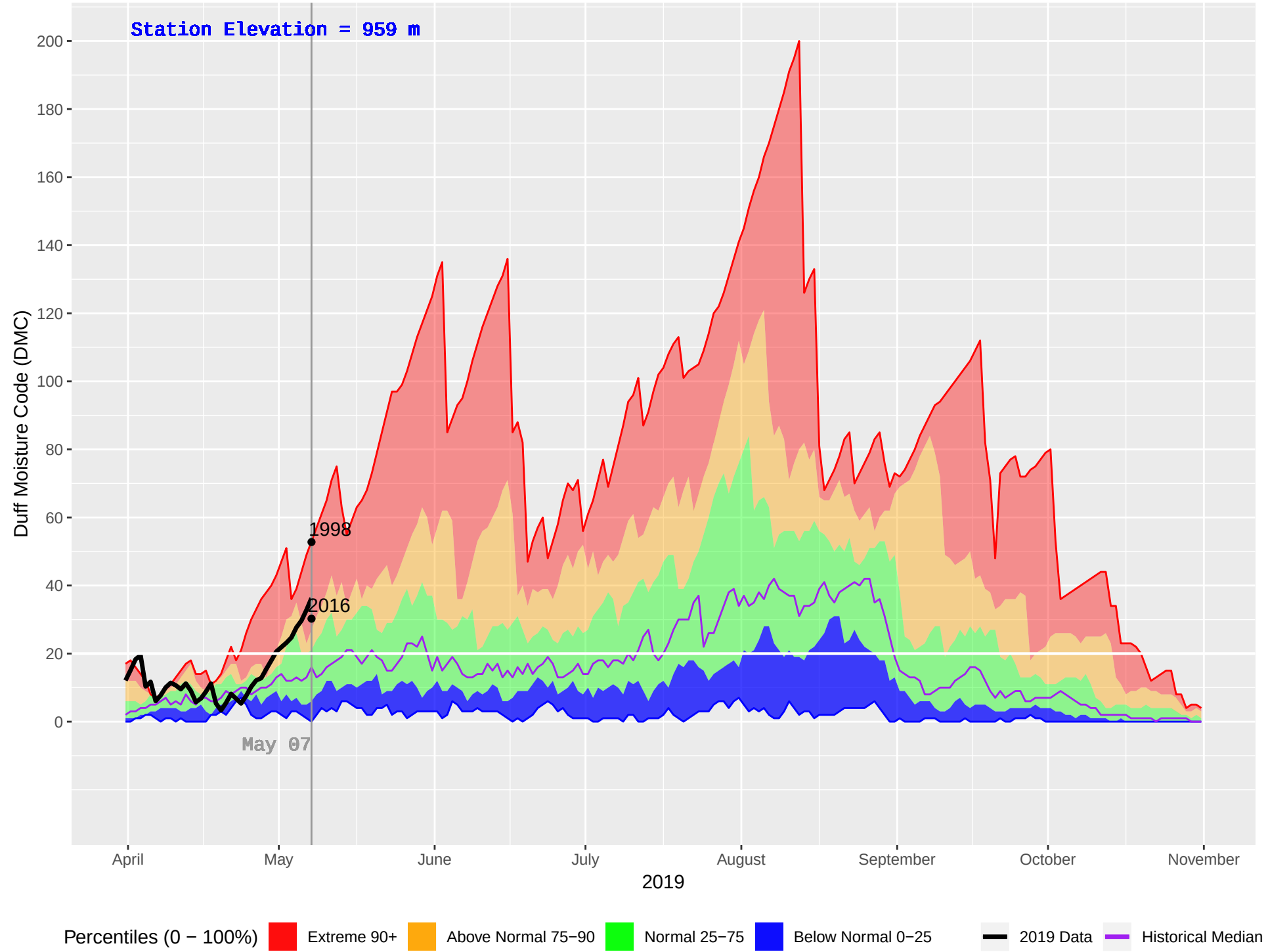
WELLS GRAY (266) : Historical (1994–2018), Current (2019) Daily Duff Moisture Code (DMC)
