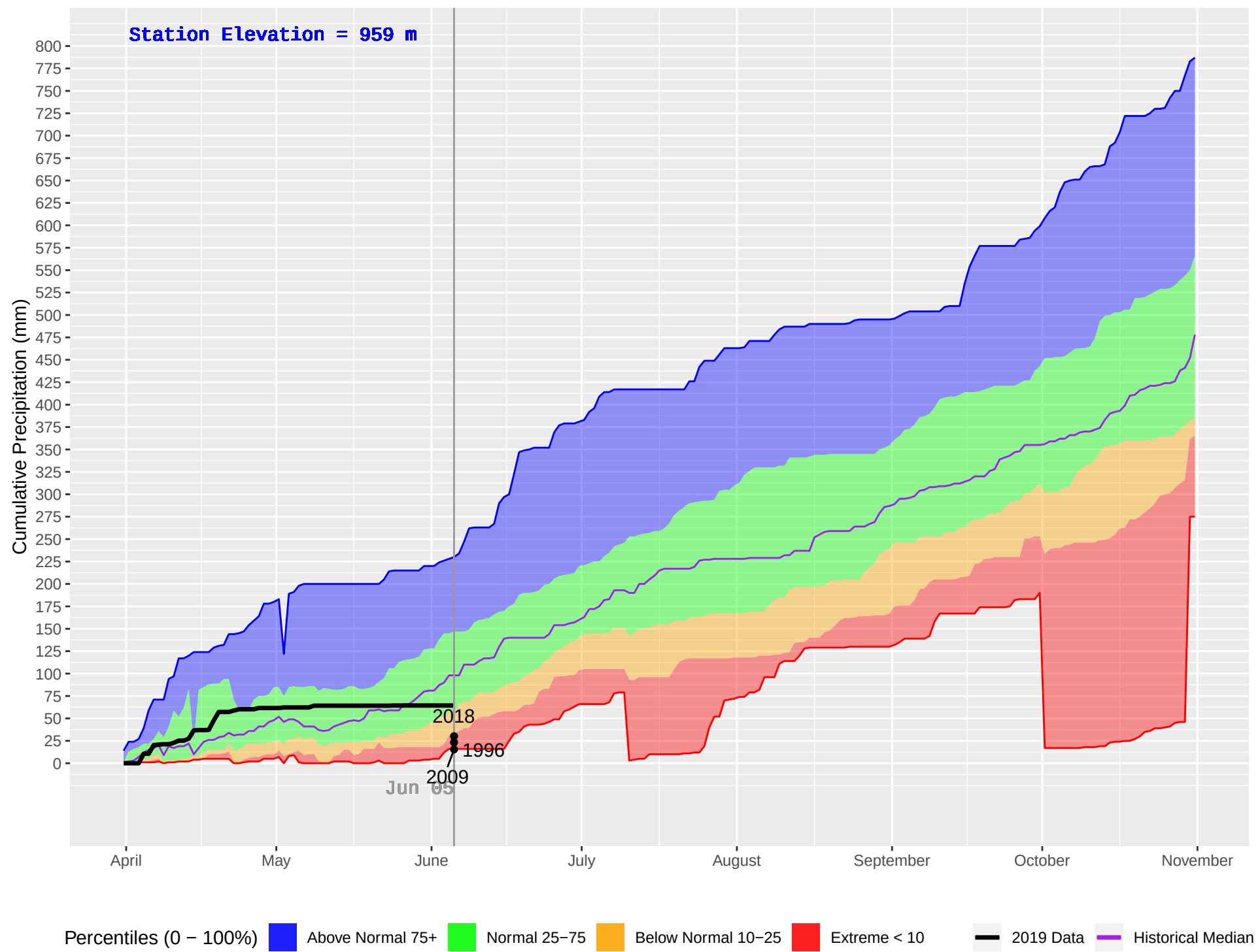
WELLS GRAY (266) : Historical (1994–2018), Current (2019) Daily Cumulative Precipitation
