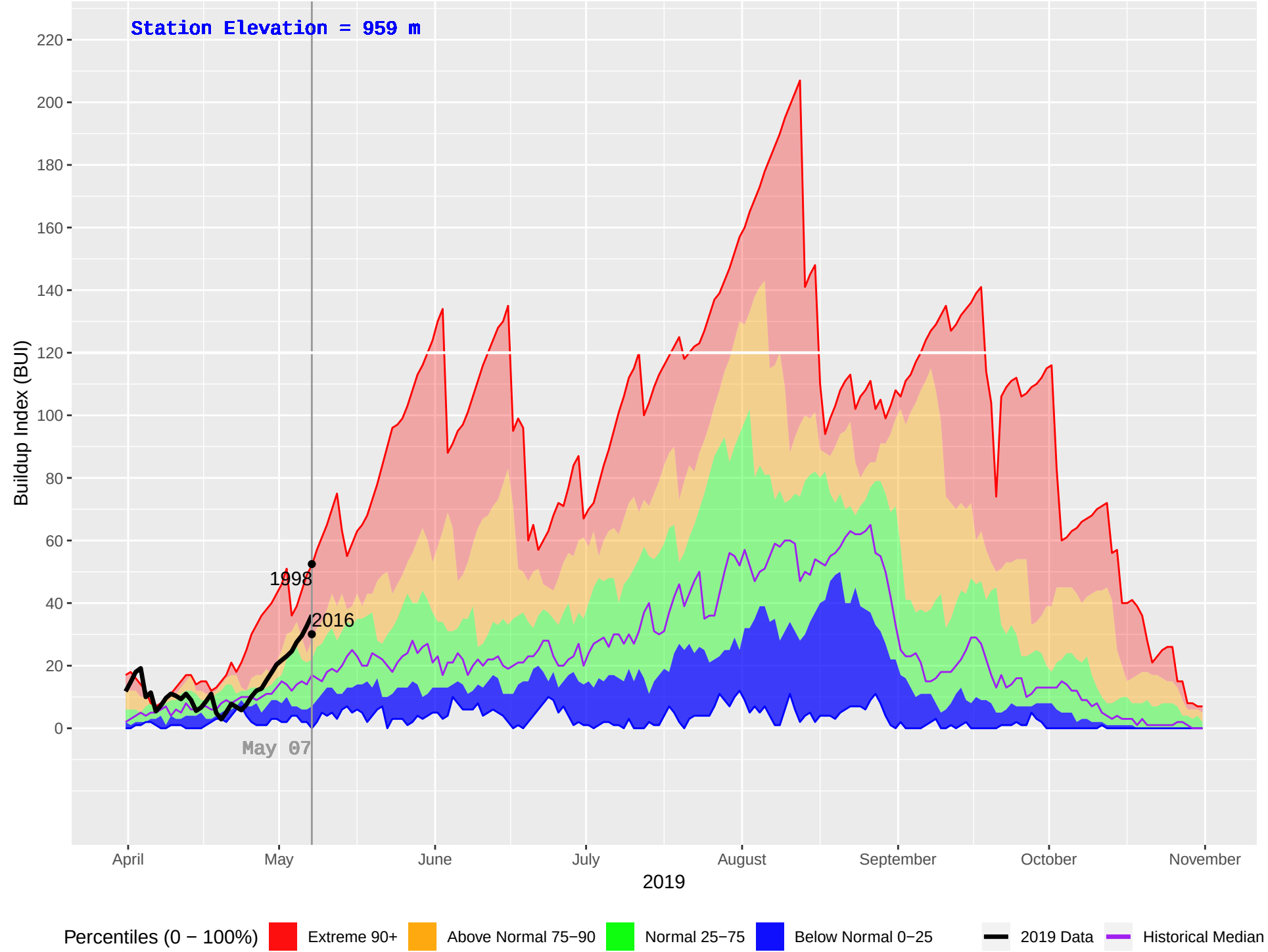
WELLS GRAY (266) : Historical (1994–2018), Current (2019) Daily Buildup Index (BUI)
